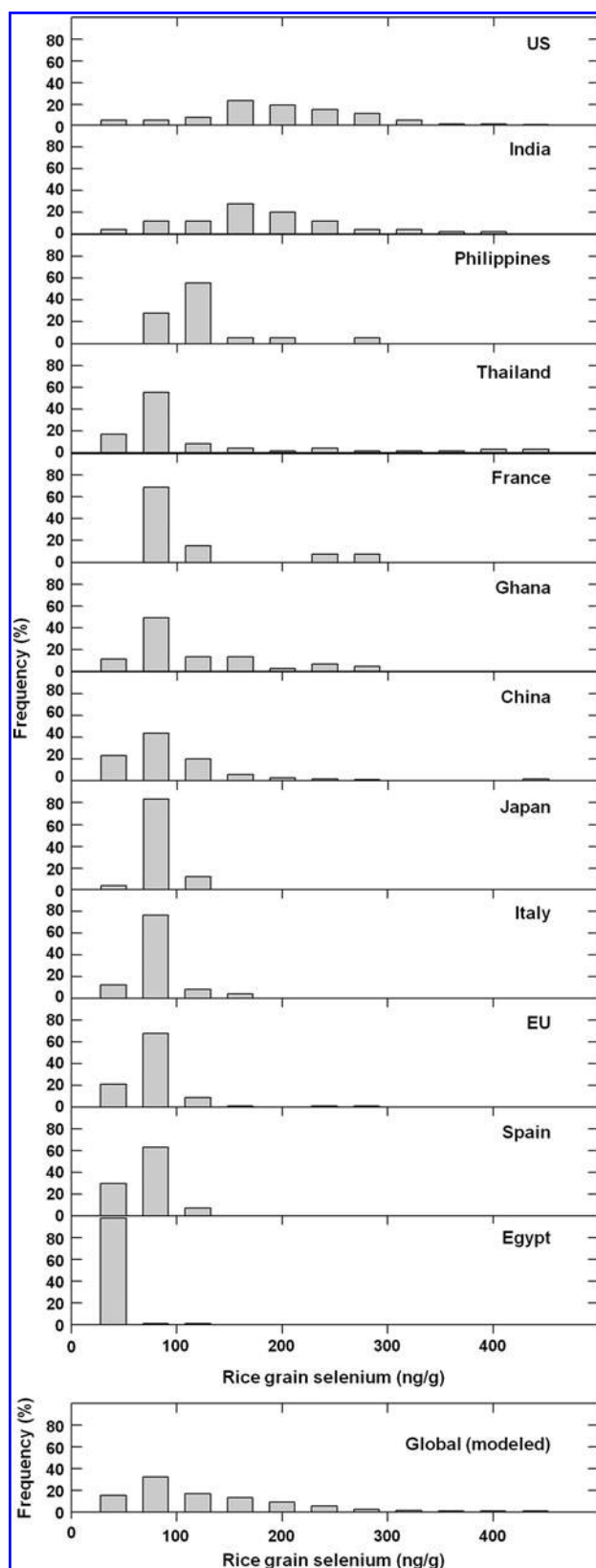
FIG. 6. Selenum content in rice produced from different countries. Selenum concentration of white (polished) rice from market stores between 2005 and 2008, from countries representing 61.5% of production and 71.1% export pools globally. Redrawn from Williams et al. (403). Data are given as percentage frequency distributions from a sample size n = 1092 .
